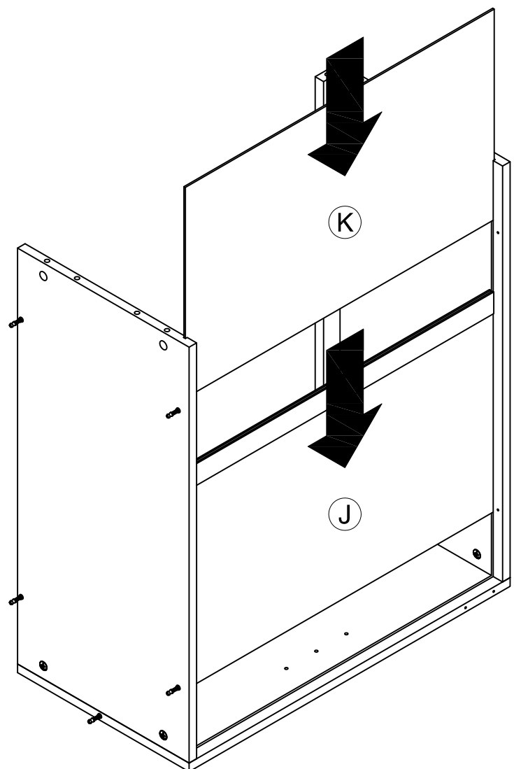
Slide Left and Right Back Panels (J) and (K) into the groove of unit.
